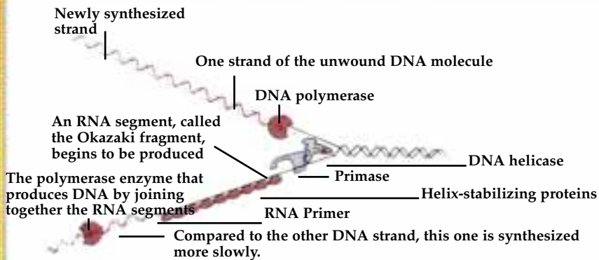
Figure 2.8 The organization of the enzymes (proteins) that work during the process of replication. Differently structured enzymes with different duties clamp together and work as a team. The DNA helicase enzyme (in the center of the diagram) unzips the DNA molecule. DNA polymerase then adds the correct nucleotides to the incomplete strand of DNA left over at the top, synthesizing a new DNA molecule. The DNA polymerase moves continuously along the top strand while the DNA is being copied. Because the other DNA strand is an exact mirror image of the initial one, the polymerase enzyme working on this strand needs to move in the opposite direction.
