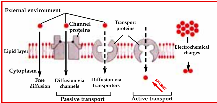
Figure 6.3 On the surface of the membrane, different gates allow different substances to be taken into the cell with the help of different enzymes. Generally, there are two types of protein gates: The first use energy for transport (active transport), selecting the necessary substances and transferring them in or out of the cell.
