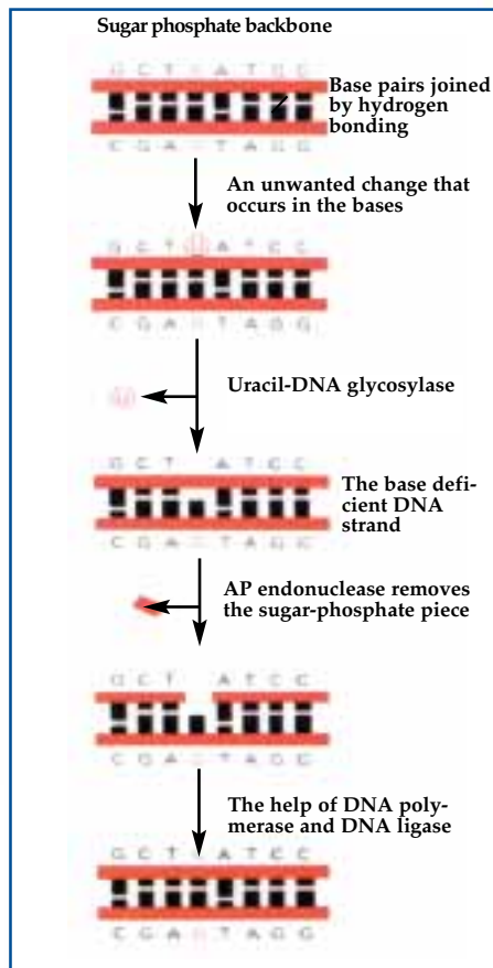
Figure 2.12 An unwanted event that occurs from time to time: the incorrect copying of the DNA molecule. As can be seen in the first diagram, a uracil (U) has been placed instead of a cytosine (C) in the fourth base position of the DNA. An enzyme called Uracil-DNA glycosylase, which has the duty of repairing only this type of mistake, removes the uracil from the DNA strand. AP endonuclease removes the sugar phosphate group from this area. DNA polymerase and DNA ligase then attach the relevant nucleotides in their place.
