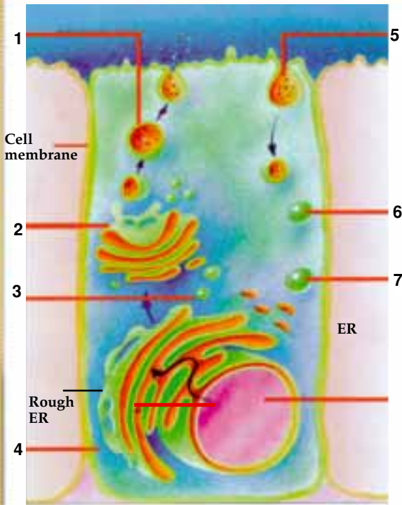
Figure 4.3 Proteins are built according to DNA instructions. In the nucleus, synthesized RNA receives from the DNA the relevant instructions needed for protein synthesis. It takes these instructions to the ribosomes and carries out protein synthesis on these organelles. Proteins synthesized on ribosomes found on the surface of the endoplasmic reticulum are deposited at the endoplasmic reticulum for transport.
