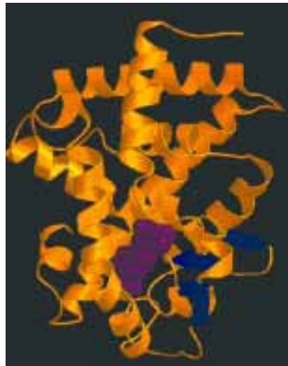
The structure of a thyroid hormone
