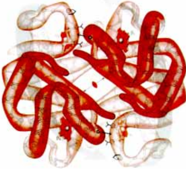
Figure 5.2 The structure of the oxyhemoglobin protein
