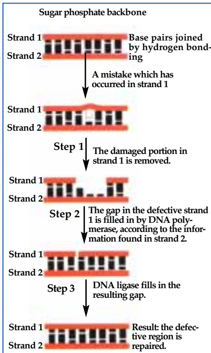
Figure 2.11 DNA control mechanisms identify and repair any mistakes arising in the DNA as a result of external factors. These mechanisms are made up of enzymes produced according to instructions found within the DNA itself. There may be different types of repair mechanisms, but basically, the damaged nucleotide is repaired according to information contained in the opposite strand's corresponding nucleotide. This process shown in the figure above basically consists of three steps: 1) After being identified by an enzyme called DNA nuclease, the damaged portion of the DNA strand is removed. This results in a gap in the DNA strand. 2) Another enzyme, DNA polymerase, adds the necessary nucleotide according to the information contained in the undamaged strand of DNA. 3) The repair of the DNA is not quite finished. The gap resulting in the sugar phosphate backbone from this repair mechanism is filled in by an enzyme called DNA ligase.
