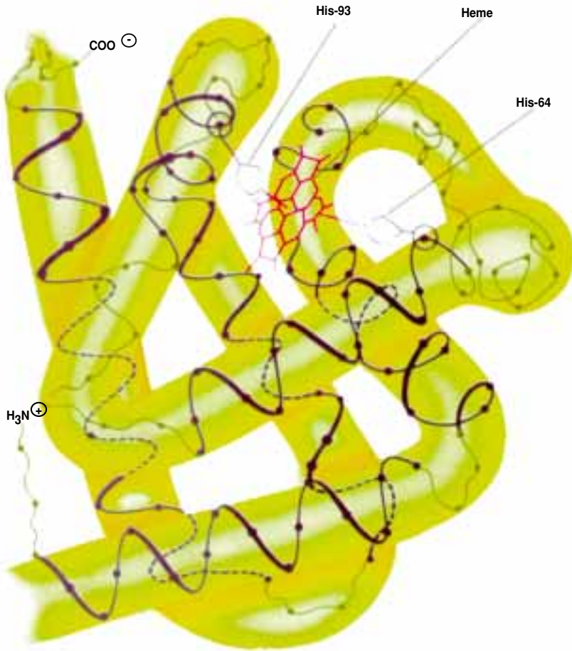
Figure 5.9 3-D shape of the myoglobin protein
