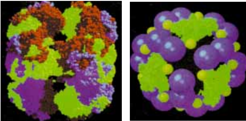
Figure 8.7 Diagrams showing the different forms of the pyruvate dehydrogenase enzyme from a bacterium called A. vinelandii . This enzyme acts on pyruvic acid formed at the end of glycolysis.
