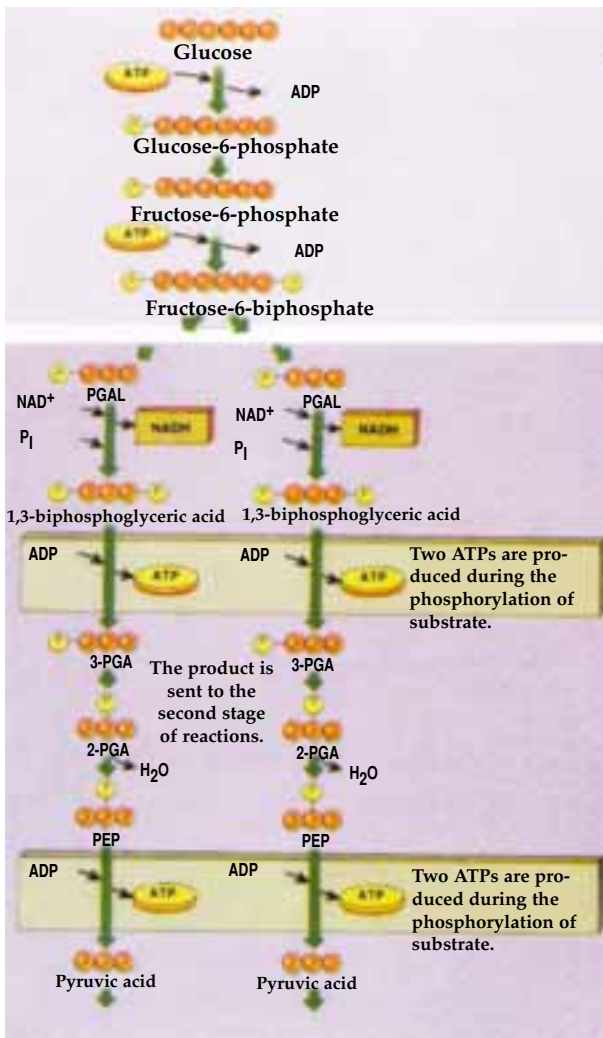
Figure 8.3 The first steps of glycolysis start with an input of energy; without energy the reaction cannot start. Enzymes transfer two phosphate groups from ATP to glucose, thereby initiating its change.
