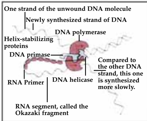
Figure 2.9 Enzymes work together in the base pairing of DNA. This combined structure resembles a sewing machine, composed of proteins, that works on the DNA from start to finish and produces a copy of it. Right: This collective mechanism in its active state. In reality, the structure shown in this figure is three-dimensional.
